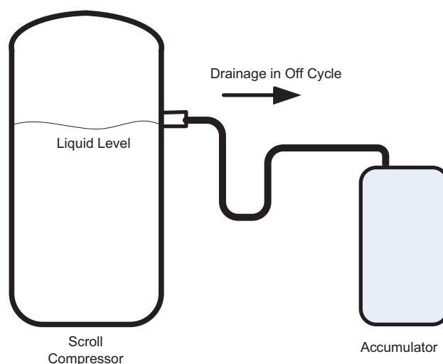
FIGURE 3: Accumulator Field Piping
